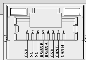
X5 CAN/RS485 (2x RJ45 standard)
